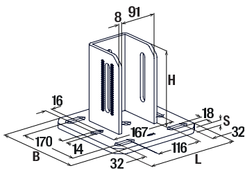
FMSF 120S
