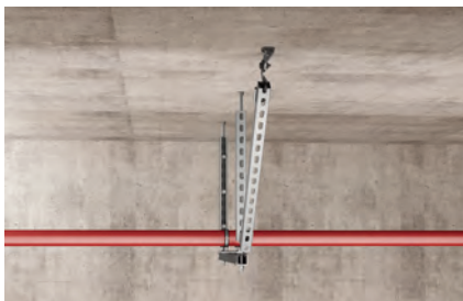
Rod stiffening for vertical seismic support
