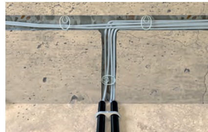
Cable fixing in wall slots < 55 mm
