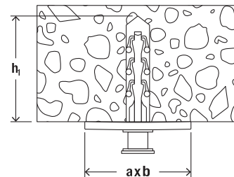
Connection piece SHA KP
