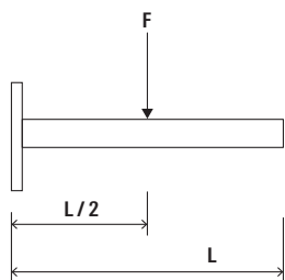
Load case 1
