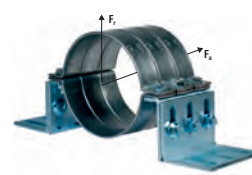
Fixpoint 3 clamps Max. recom. load axial F_a = 16500 N radial F_r = 13980 N
