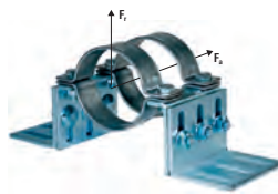
Fixpoint 2 clamps Max. recom. load axial F_a = 11000 N radial F_r = 9320 N
