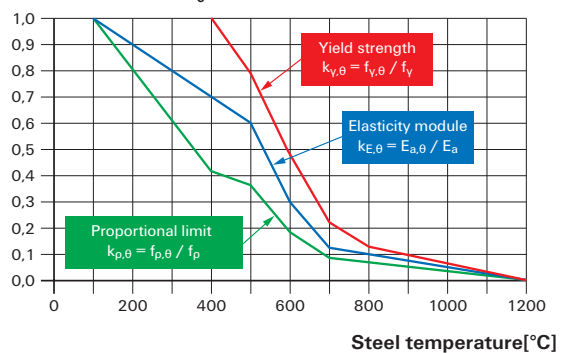
Dependency of the yield strength, proportional limit and elasticity module on the temperature (basis: EN1993-1-2:2012-12 Eurocode 3).
