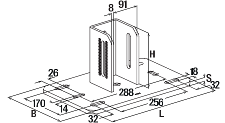
FMSF 120L
