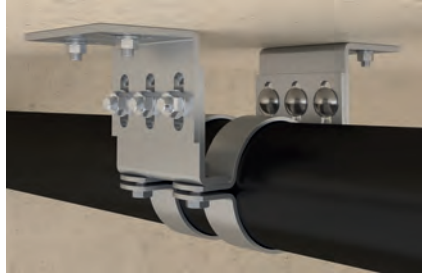
Fixpoint-pipecollar
