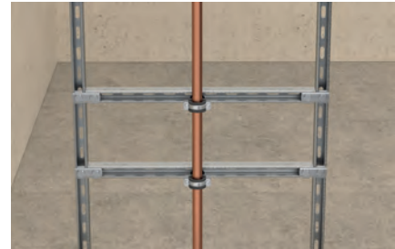
Vertical installation
