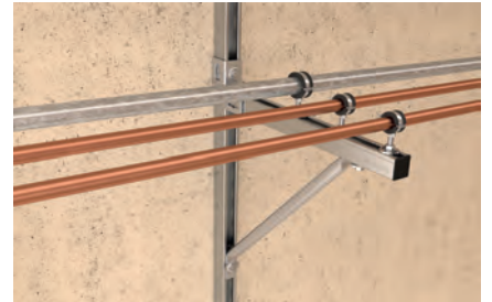
Leightweight installation on cantilever
