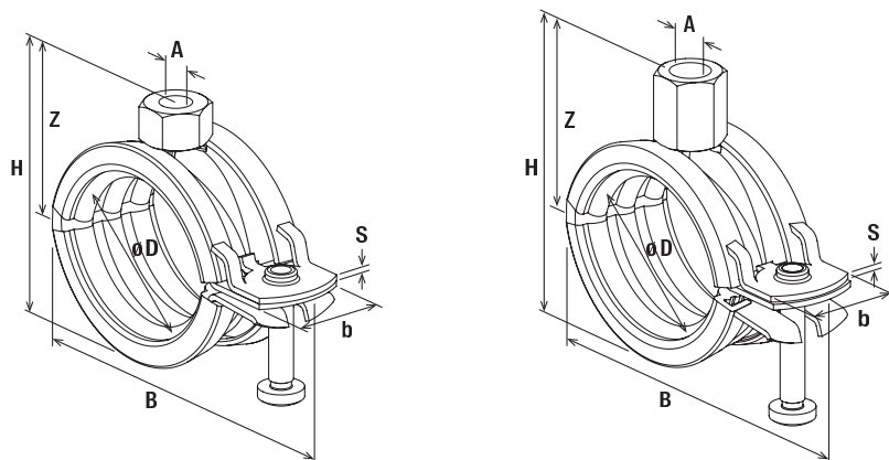
FGRS Plus
