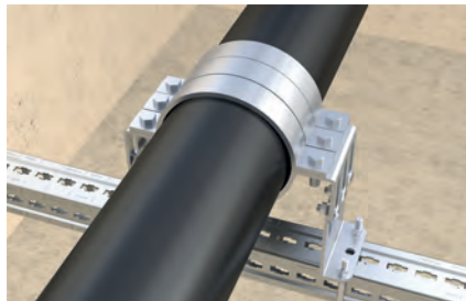
Fix-point clamp construction
