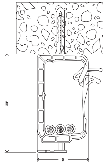
Installation base SHA MS
